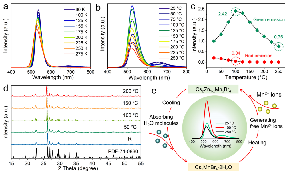
Fig. 3 (a) Temperature-dependent PL spectra of Cs 2 ZnBr 4 :25%Mn 2+ sample 365 nm upon excitation along with temperature range from 80 to 275 K. (b) Temperature-dependent PL spectra of Cs 2 ZnBr 4 :25%Mn 2+ sample upon 365 nm excitation along with temperature range from RT to 250 °C. (c) Normalized integrated PL intensities of green and red emissions in Cs 2 ZnBr 4 :25%Mn 2+ sample at different temperatures. (d) Temperature-dependent in situ PXRDs of Cs 2 ZnBr 4 :25%Mn 2+ sample along with temperature range from RT to 200 °C (e) Schematic illustration for unusual PL thermal enhancement process in Mn 2+ -doped Cs 2 ZnBr 4 samples.
