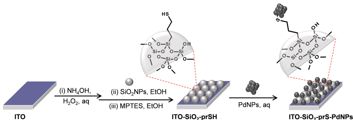
Scheme 1 Step-by-step fabrication of ITO-SiO 2 -prS-PdNPs as described in Section 2.5.
