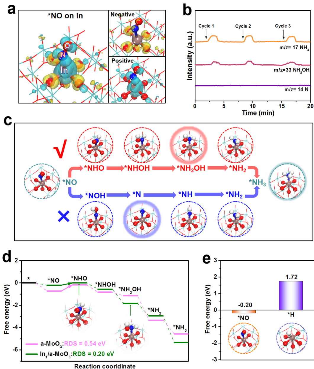
Fig. 4 (a) Charge density difference of absorbed NO (*NO) on \text{In}_1/\text{a-MoO}_3 . Yellow and cyan regions represent electron depletion and accumulation, respectively. (b) Online DEMS spectra of \text{In}_1/\text{a-MoO}_3 during the electrolysis at -0.6 V. (c) Schematic of typical NOH and NHO pathways on \text{In}_1/\text{a-MoO}_3 . (d) Free energy profiles of the NORR process (NHO pathway) on the Mo site ( \text{a-MoO}_3 ) and In site ( \text{In}_1/\text{a-MoO}_3 ). (e) Binding free energies of *NO and *H on the In site of \text{In}_1/\text{a-MoO}_3 .
