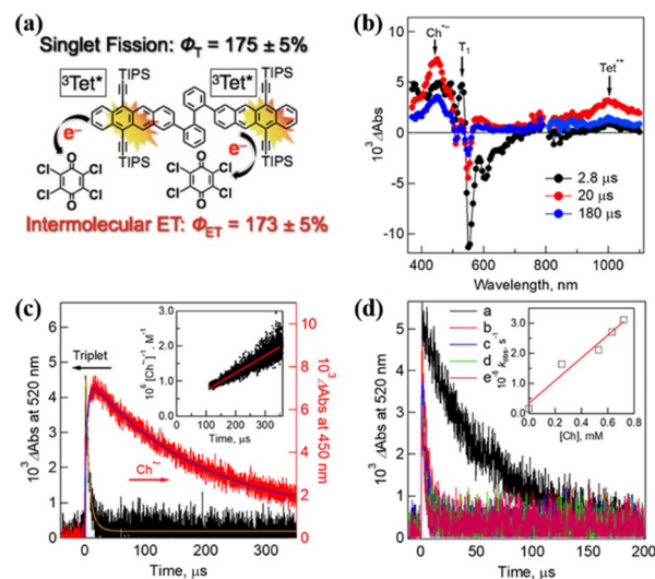
Fig. 18 (a) Schematic diagram of intermolecular electron transfer from iSF of tetracene dimer 14 to chloranil. (b) \mu\text{s} -TA spectra of dimer 14 ( 50 \mu\text{M} ) in the presence of 250 \mu\text{M} chloranil in Ar-saturated PhCN after excitation at 532 \text{ nm} . (c) Time profiles of absorption at 520 \text{ nm} in the presence of different concentrations of chloranil: (a) 0 \text{ mM} , (b) 0.25 \text{ mM} , (c) 0.53 \text{ mM} , (d) 0.63 \text{ mM} , and (e) 0.72 \text{ mM} . The inset shows the plot of the pseudo-first-order rate constant ( k_{\text{obs}} ) vs. the concentration of chloranil. Reproduced with permission. 75 Copyright 2019, the American Chemical Society.
