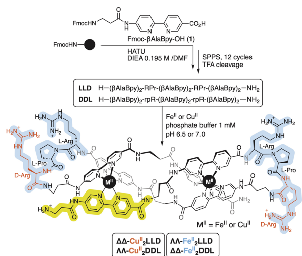
Scheme 1 Sequences of the peptide ligands LLD and DDL equipped with six units of the Fmoc- \beta\text{AlaBpy-OH} ( 1 ) coordinating residue. After their synthesis by SPPS methods, cleavage, and purification, the Cu II helicates are stereoselectively folded under thermodynamic control in the presence of Cu II ions. L-amino acids are indicated in upper-case, and D-amino acids in lower case ( i.e. , R, P for L-Arg and L-Pro, and r for D-Arg). Heterochiral \beta -turn loops are highlighted in blue and one of the six coordinating residues ( 1 ) in yellow.
