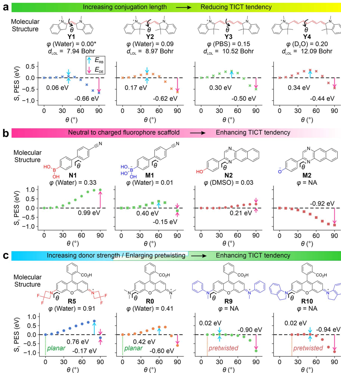
Fig. 2 Calculated S_1 PES for TICT at the (a) \omega B97XD/Def2SVP/cLR-PCM level and (b and c) CAM-B3LYP/Def2SVP/cLR-PCM level for various compounds in water. The rotation barrier ( E_{RB} ), driving energy ( E_{DE} ), experimental quantum yield ( \phi ) 12,34,35,40–44 and mean localization distance ( d_{LOL} ) are labelled in the inset. Due to the lack of experimental data, \phi of Y1 is adapted from a monomethine cyanine analog, thiazole orange. 45
