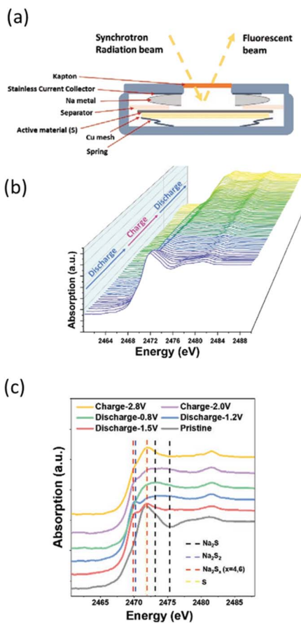
Fig. 6 (a) Scheme of coin cells allowing measuring S K-edge operando in fluorescence mode. (b) Sulfur K-edge XANES evolution as a function of the state of charge followed operando in Na/S batteries and (c) selected spectra at various states during the first cycle with positions for reference compounds highlighted by vertical dotted lines. Reproduced from ref. 19, © John Wiley & Sons.
