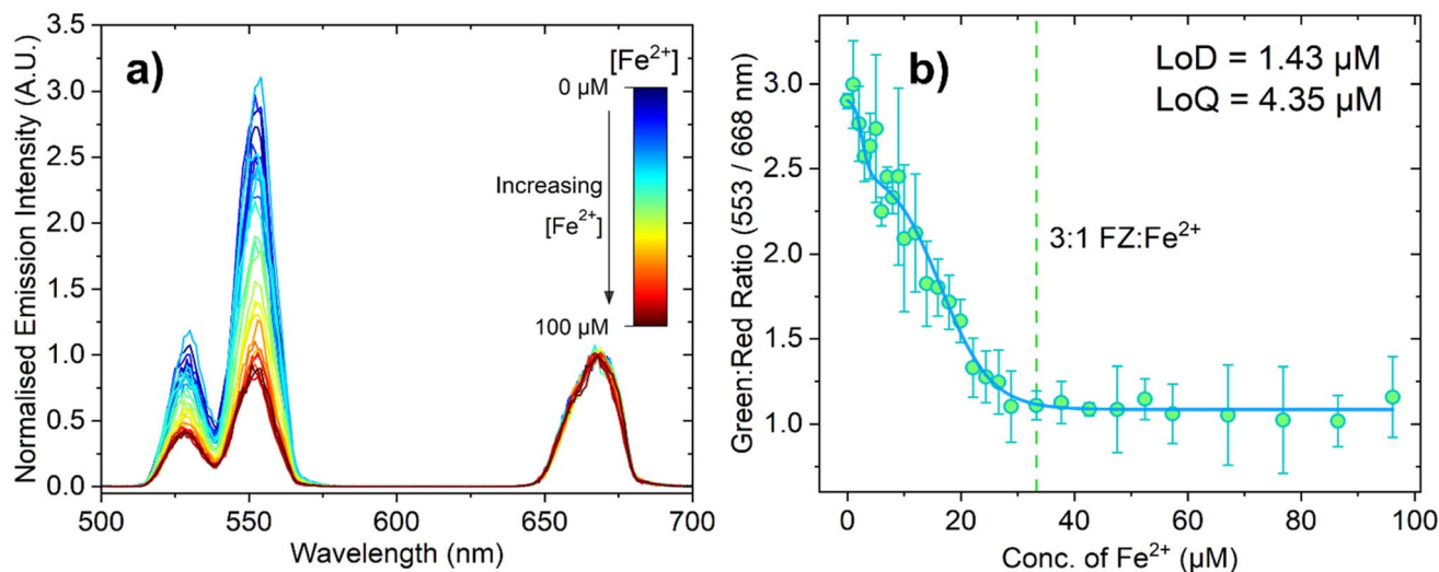
Fig. 5 (a) Emission spectrum of ferrozine (100 μM) in pH 5.6 MES buffer (0.1 M) with 150 μL NaYF 4 :Yb 3+ ,Er 3+ -doped UCNPs with increasing concentration of Fe 2+ ions. The spectra have been normalised to the peak centred at 668 nm. This spectrum shows an example of one repeat, where three repeats were conducted overall. The emission monochromator bandwidth was set to 13 nm. (b) The ratio between the intensity of the green (554 nm) and red (668 nm) peaks at each concentration of Fe 2+ , with the error bars representing standard deviation over three repeats. The green dashed line represents the concentration at which the 3 : 1 FZ:Fe 2+ complex is expected to form (33.33 μM Fe 2+ ). Data fitted using a biphasic dose response function in OriginPro®.
