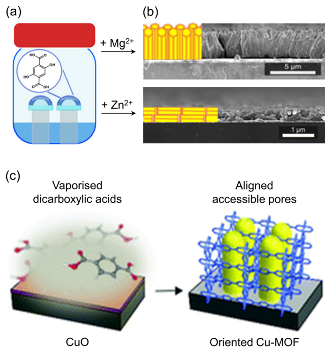
Fig. 10 (a) Schematic illustration of VAC reactions for MOF-74 films with Mg 2+ or Zn 2+ as a metal source. (b) Cross-sectional SEM images of Mg-MOF-74 film (top) and Zn-MOF-74 film (down). Adapted with permission from ref. 88. Copyright 2021, American Chemical Society. (c) Schematic illustration of the CVD process for synthesizing oriented films of CuCDC and CuBDC by reacting a deposited layer of CuO with a vaporized carboxylic acid. Adapted with permission from ref. 89. Copyright 2019, Royal Society of Chemistry.
