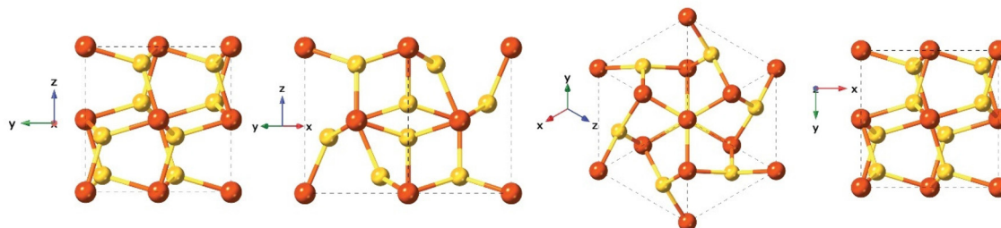
Fig. 9 Different crystal face views of the pyrite structure.
