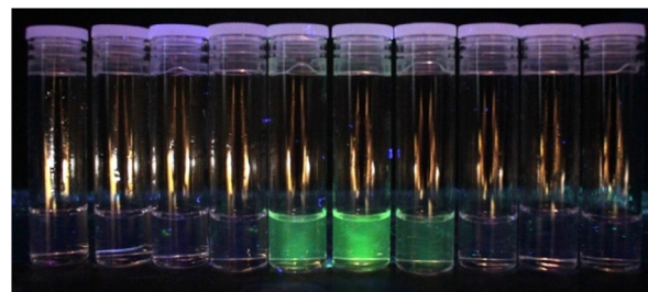
Fig. 3 Eluted GPC solvent showing the emission from the yellow (green-emissive) Nap-PA-CHO polymer in vials 5–7 ( t_R = 14 –17 min; each vial = 1 mL, i.e. 1 mL).
