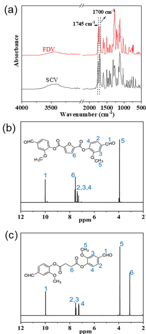
Fig. 2 FTIR spectra (a) and 1 H NMR spectra of FDV (b) and SCV (c).
