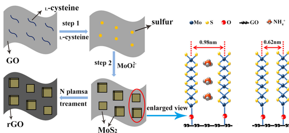
Scheme 1 Schematic illustration of the synthesis of N-rGO/ \text{MoS}_2(\text{ISE}) .
