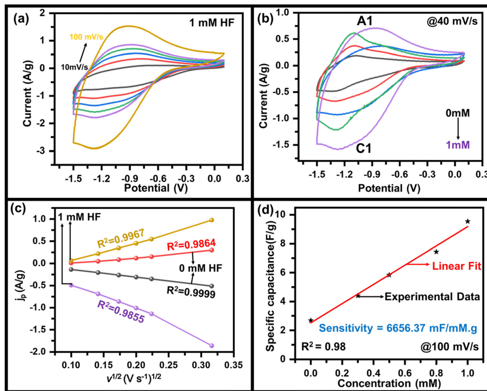
Fig. 2 CV graph of \text{MoO}_3 at GCE with (a) 1 mM HF, (b) 0 mM, 0.2 mM, 0.5 mM, 0.8 mM, and 1.0 mM HF in 0.5 M \text{LiClO}_4 in PC, (c) variation of current density ( j_p ) vs. v^{1/2} graph with and without HF, and (d) variation of specific capacitance with concentration of HF including raw data and linear fit.
