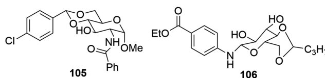
Fig. 65 D-Glucosamine amide and alkyl derivatives as gelators.
