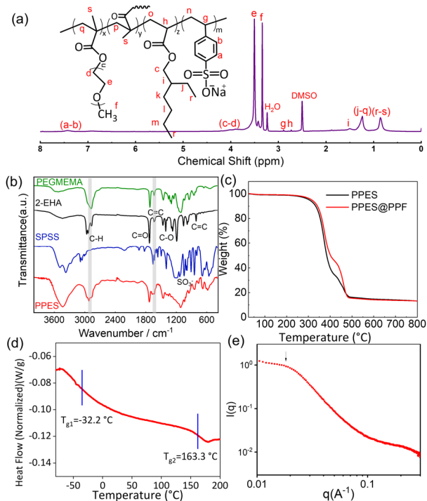
Fig. 1 Characterization studies of monomers and the as-prepared polymer. (a) 1 H NMR spectra of the prepared PPES. (b) FT-IR spectra of PEGMEMA, 2-EHA, SPSS, 2-EHA monomers and the resulting polymer network PPES. (c) The thermogravimetric analysis of PPES and PPES@PPF. (d) DSC curve of PPES. (e) SAXS spectrum of PPES.
