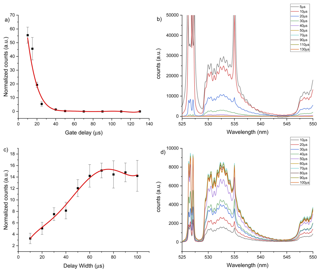
Fig. 2 LIBS signal optimization under argon flow of 1 \text{ L min}^{-1} for 530 nm window using a 2500 \mu\text{g g}^{-1} hydroxyapatite standard. (a) Gate delay optimization maintaining constant gate width at 50 \mu\text{s} , (b) LIBS spectrum for each gate delay change, (c) gate width optimization maintaining constant gate delay at 20 \mu\text{s} , (d) LIBS spectrum for each gate width change.
