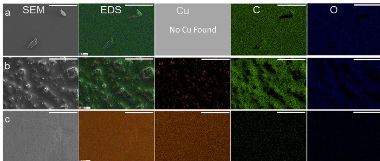
Fig. 3 SEM/EDX images at 500 \times magnification for (a) -560 mV RHE fouled Cu (used three times), (b) -700 mV RHE fouled Cu (used three times), (c) bare Cu. Scale bar shown is 100\ \mu\text{m} for all images. Columns from left to right are labeled on top row.
