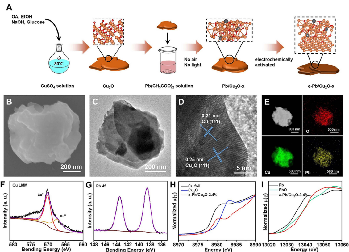
Fig. 1 (A) Schematic illustration of the preparation of e- \text{Pb/Cu}_2\text{O-}3.4\% . (B) SEM image of e- \text{Pb/Cu}_2\text{O-}3.4\% . (C and D) TEM and HRTEM images of e- \text{Pb/Cu}_2\text{O-}3.4\% . (E) Elemental mappings of e- \text{Pb/Cu}_2\text{O-}3.4\% . (F) Cu LMM XPS spectra of e- \text{Pb/Cu}_2\text{O-}3.4\% . (G) Pb 4f XPS spectra of e- \text{Pb/Cu}_2\text{O-}3.4\% . (H) Cu K-edge XANES spectra of e- \text{Pb/Cu}_2\text{O-}3.4\% . (I) Pb L-edge XANES spectra of e- \text{Pb/Cu}_2\text{O-}3.4\% .
