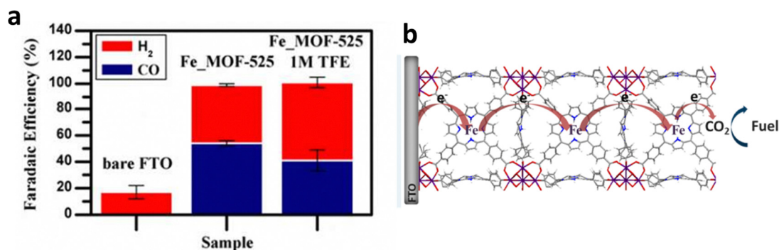
Fig. 19 (a) FE over approximately 4 h of bare FTO, Fe_MOF-525 with/without 2,2,2-trifluoroethanol (TFE). (b) Proposed ECR mechanism on the Fe porphyrin-based MOF. Reproduced with permission. 22 Copyright (2015) American Chemical Society.
