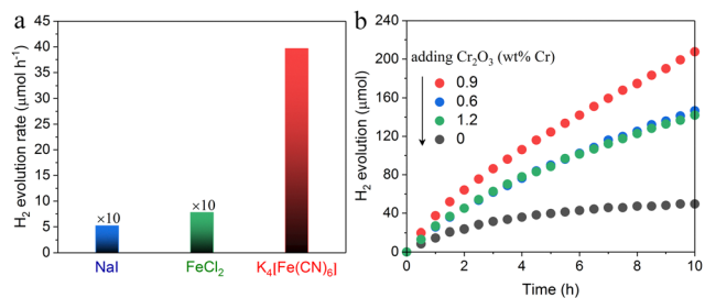
Fig. 6 (a) Photocatalytic \text{H}_2 evolution activities of \text{Cr}_2\text{O}_3/\text{Na-Pt}/\text{BaTaO}_2\text{N:Zr0.01} ( 100\text{ mg} ) in aqueous solutions of NaI, \text{FeCl}_2 and \text{K}_4[\text{Fe}(\text{CN})_6] ( 150\text{ mL} , 2\text{ mM} each) with pH values of 6–7, 2.3 and 6, respectively. (b) Time courses of \text{H}_2 evolution over \text{Cr}_2\text{O}_3/0.23\text{ wt\% Na} 0.3\text{ wt\% Pt}/\text{BaTaO}_2\text{N:Zr0.01} ( 100\text{ mg} ) with varying amounts of Cr in an aqueous 50\text{ mM} sodium phosphate buffer solution at pH 6 ( 150\text{ mL} ) containing 6\text{ mM} \text{K}_4[\text{Fe}(\text{CN})_6] . Light source: 300\text{ W} xenon lamp ( 420\text{ nm} < \lambda < 800\text{ nm} ).
