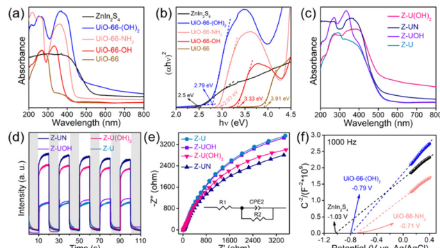
Fig. 5 UV-vis DRS (a) and (\alpha hv)^2 versus h\nu curves (b) of ZnIn 2 S 4 , UiO-66-(OH) 2 , UiO-66-NH 2 , UiO-66-OH and UiO-66, UV-vis DRS (c), photocurrent spectra (d) and EIS Nyquist plots (e) of Z-UN, Z-U(OH) 2 , Z-UOH and Z-U, Mott-Schottky plots of ZnIn 2 S 4 , UiO-66-(OH) 2 and UiO-66-NH 2 (f).
