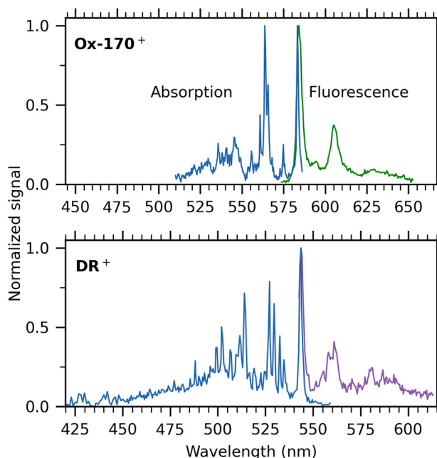
Fig. 5 100 K absorption spectra (blue) based on fluorescence-excitation experiments and dispersed-fluorescence spectra of gaseous \text{Ox-170}^+ (top) and \text{DR}^+ (bottom). The same energy range has been used for both spectra to enable easy comparison of the widths of the spectra. Excitation wavelengths to measure fluorescence spectra were 561 nm ( \text{Ox-170}^+ ) and 532 nm ( \text{DR}^+ ). The main absorption bands are saturated resulting in an incorrect intensity relation between the main band and the rest of the spectrum. The relatively high laser power ( <0.1 mW) was used to enable measurement of the vibrational structure.
