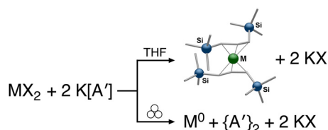
Fig. 7 Reaction of \text{MX}_2 ( \text{M} = \text{Cr}, \text{Fe}, \text{Co} ) with \text{K}[\text{A}'] in THF produces the intended [\text{MA}'_2] complexes via halide metathesis. Grinding the reagents together without solvent leads to a redox process with metal reduction and ligand coupling.
