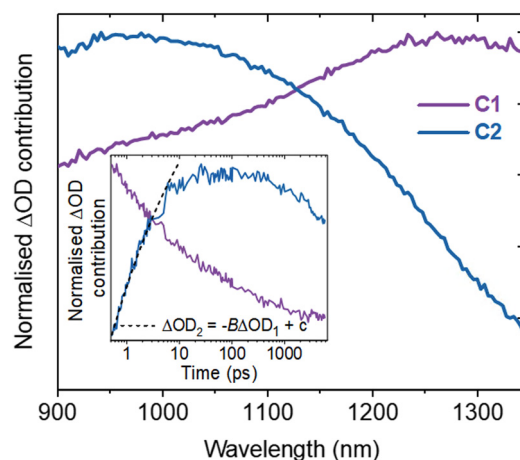
Fig. 2 Spectral deconvolution of the NIR region to extract two components. Inset shows a comparison of the normalised C1 and C2 kinetics at 0.40 mJ cm -2 by kinetic analysis, including fitting the optical signal of C1 ( \Delta OD_1 ) to C2 ( \Delta OD_2 ).
