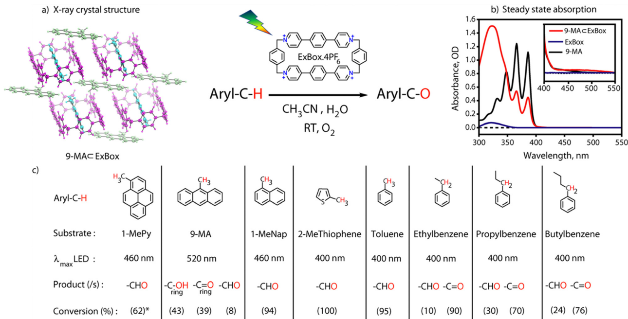
Fig. 2 (a) Single crystal structure of 9-MA \subset ExBox 4+ ; (b) steady state absorption spectra of 9-MA, ExBox 4+ and 9-MA \subset ExBox 4+ showing formation of CT states; (c) visible light mediated photoreaction scheme for sp 3 C–H bond functionalization, where 2.5 mM ExBox and 2–3 equiv. of guests are used, photoreaction time = 24 hours (72 hours for Toluene), LED light intensity: 50–175 mW cm -2 , and product conversions are obtained from GCMS, * from 1 H NMR.
