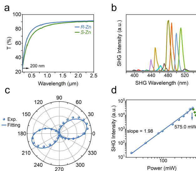
Fig. 2 (a) UV-vis-NIR transmittance spectra of R/S-Zn . (b) Wavelength-dependent SHG intensities of R-Zn at various excitation wavelengths from 800 to 1040 nm. (c) Polarization dependence of the SHG intensity from the R-Zn crystal under the excitation of 960 nm. (d) Logarithmic plot of SHG intensity as a function of the incident power.
