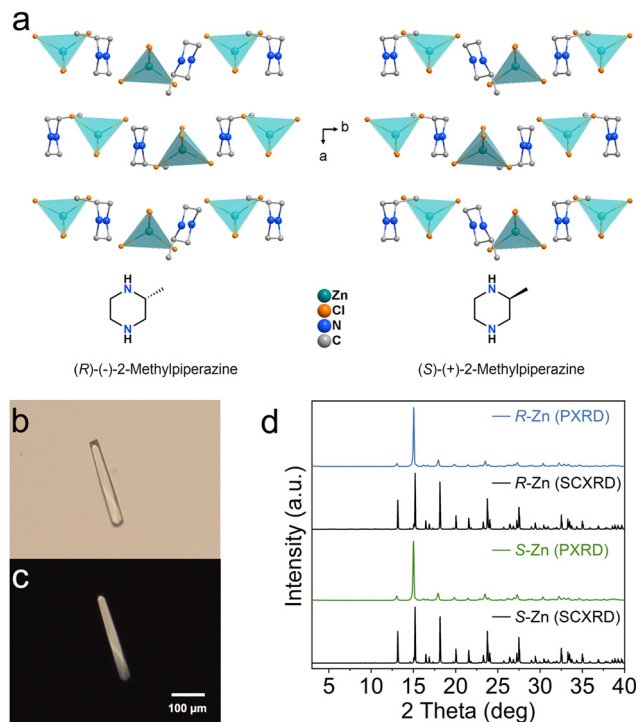
Fig. 1 (a) Crystal structures of R - and S - Zn . (b) Optical microscope image and (c) the corresponding crossing polarized microscope image of an R - Zn crystal. (d) Powder XRD patterns of R - and S - Zn .
