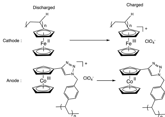
Scheme 10 Electrode reactions in a recent RFBs based on ferrocene polymer as catholyte and cobaltocenium salt as anolyte (driving force: 1.3 V). Electrons are transported by ClO 4 - anions.
