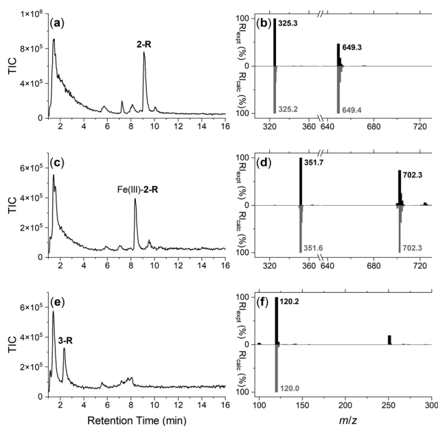
Fig. 1 LC-MS traces reported as total ion current (TIC) from the eluent from a TCEP wash of the (a) DFOB-SS-Resin (2-R), (c) Fe(III)-DFOB-SS-Resin (Fe(III)-2-R), or (e) MA-SS-Resin (3-R), with experimental (black) MS signals from the peak at (a) 9.1 min, (c) 8.3 min, or (e) 2.4 min in (b), (d) or (f), respectively, with calculated signals ( [M + 2H]^{2+} and/or [M + H]^+ adducts) for DFOB-SH (2), Fe(III)-DFOB-SH (Fe(III)-2) or MA-SH (3) in grey.
