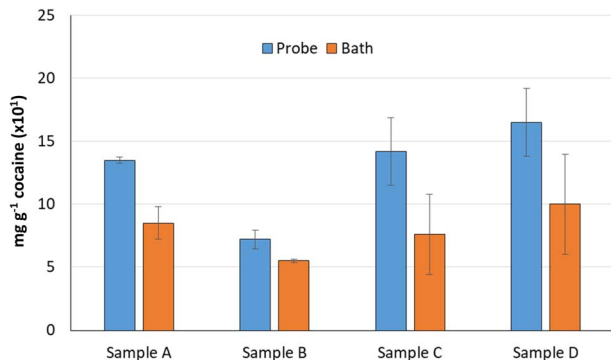
Fig. 3 Comparison of cocaine amount extracted of four seized samples ( n = 3 ) by employing the proposed ultrasound probe extraction (4 mL ethanol, 60% power, 1 minute extraction time, continuous mode) and ultrasound water bath extraction (4 mL ethanol and 75 minutes extraction time).
