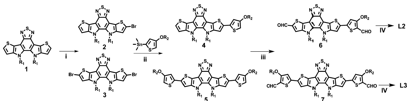
Scheme 1 Synthetic routes to L2 and L3 . (i) NBS, THF, 0 °C; (ii) (4-((2-hexyldecyl)oxy)thiophen-2-yl)trimethylstannane, \text{Pd}(\text{PPh}_3)_4 , toluene, reflux; (iii) \text{POCl}_3 , 1,2-dichloroethane, DMF, 80 °C; (iv) 2-(5,6-difluoro-3-oxo-2,3-dihydro-1H-inden-1-ylidene)malononitrile, pyridine, \text{CHCl}_3 , rt.
