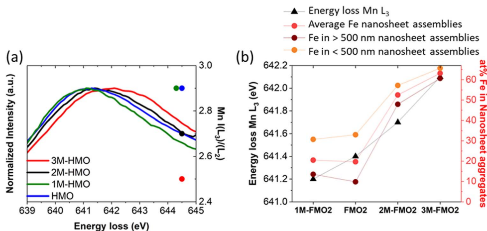
Fig. 8 (a) Left-Y Axis: EELS \text{Mn } L_3 peaks of HMO, 1M-HMO, 2M-HMO and 3M-HMO. Right-Y axis: corresponding \text{Mn } (L_3)/(L_2) values. (b) Trends of oxidation state of x\text{M-HMO} (Left-Y axis) and Fe introduced by galvanic exchange reaction (right-Y axis) for x\text{M-FMO2} .
