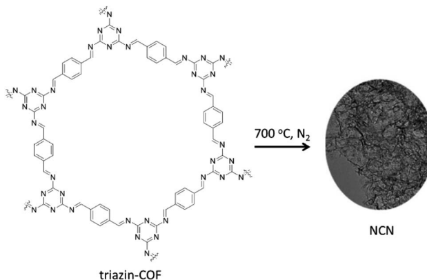
Fig. 15 Carbonization of triazine–COF to NCN.
