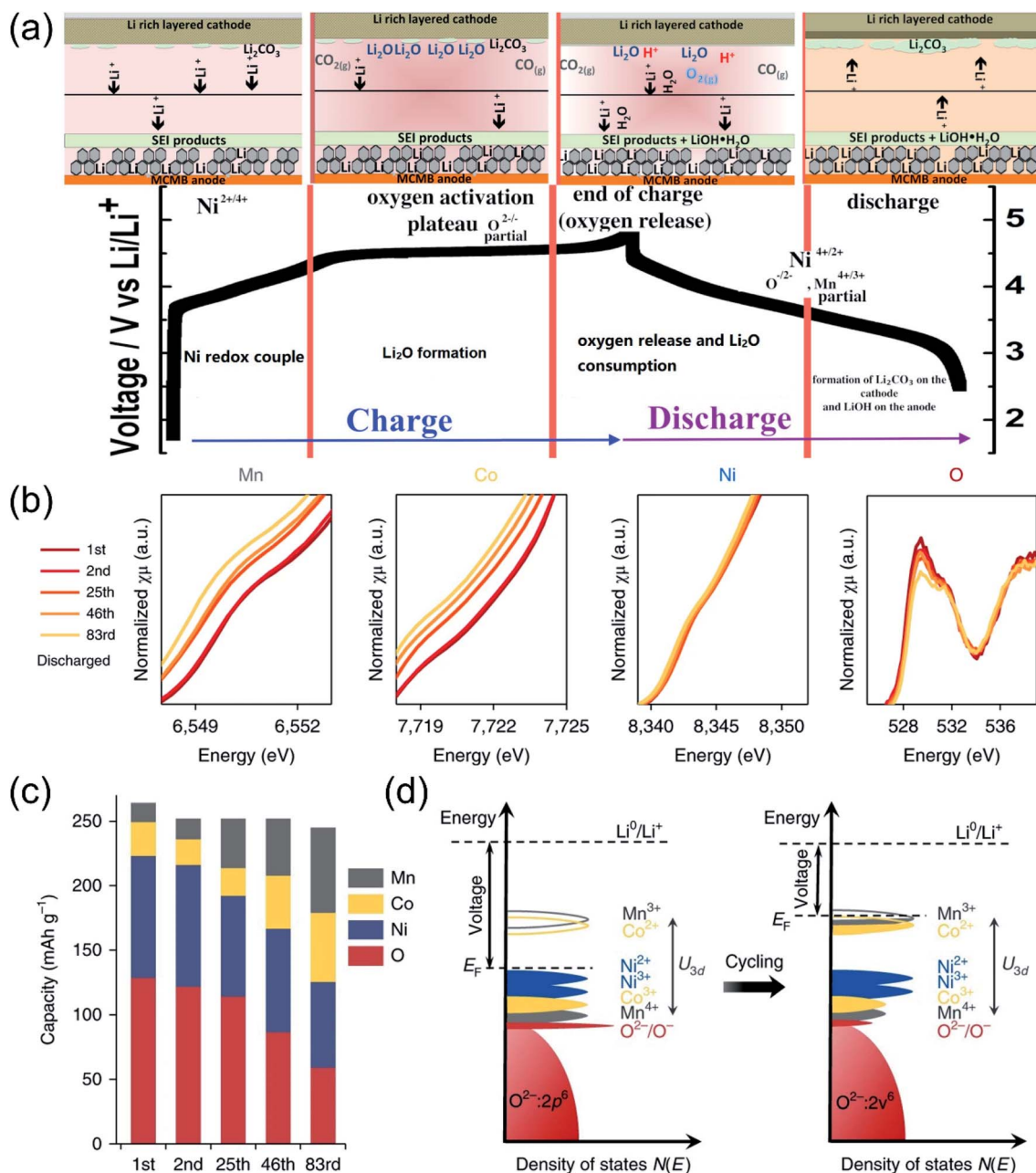
Fig. 3 Proposed redox reaction of Li[Ni_xLi_{(1-2x)/3}Mn_{(2-x)/3}]O_2 for oxygen activating members during the charging and discharging process. Reproduced with permission from ref. 43. Copyright 2014, the American Chemical Society. (b) K-edge XAS of Mn, Co, Ni and O for Li_{1.2}Ni_{0.15}Co_{0.1}Mn_{0.55}O_2 collected after the 1st, 2nd, 25th, 46th and 83rd cycles. For transition metals (Mn, Co and Ni), XAS is collected in the transmission mode; for oxygen, it is collected in the FY mode. (c) The contribution towards the discharge capacity from each element at various cycles. (d) An illustration of the Fermi level being lifted up as a result of electronic structure change. As the voltage is determined by the energy gap between the Fermi level and the Li^+/Li^0 energy level, it is lowered accordingly. U_{3d} is the on-site coulombic repulsion energy that splits up successive redox potentials. Reproduced with permission from ref. 10. Copyright 2018, Springer Nature.
