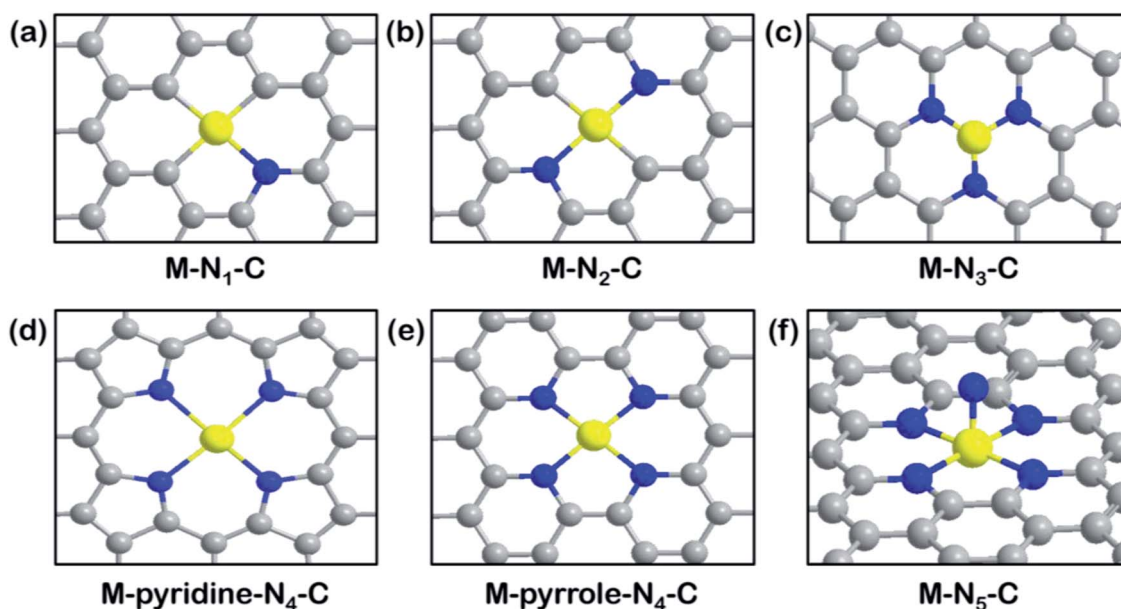
Fig. 3 Overview of M–N–C structures. Schematic illustration of (a) M-N_1-C . Reproduced with permission from ref. 86, copyright 2020, American Chemical Society. (b) M-N_2-C . Reproduced with permission from ref. 88, copyright 2019, Wiley-VCH. (c) M-N_3-C . Reproduced with permission from ref. 81, copyright 2018, Wiley-VCH. (d) M -pyridine- N_4-C . Reproduced with permission from ref. 91, copyright 2020, Springer Nature Publication. (e) M -pyrrole- N_4-C . Reproduced with permission from ref. 77, copyright 2019, Science. (f) M-N_5-C molecular models. Reproduced with permission from ref. 93, copyright 2019, Wiley-VCH. (M: yellow; C: grey; N: blue).
