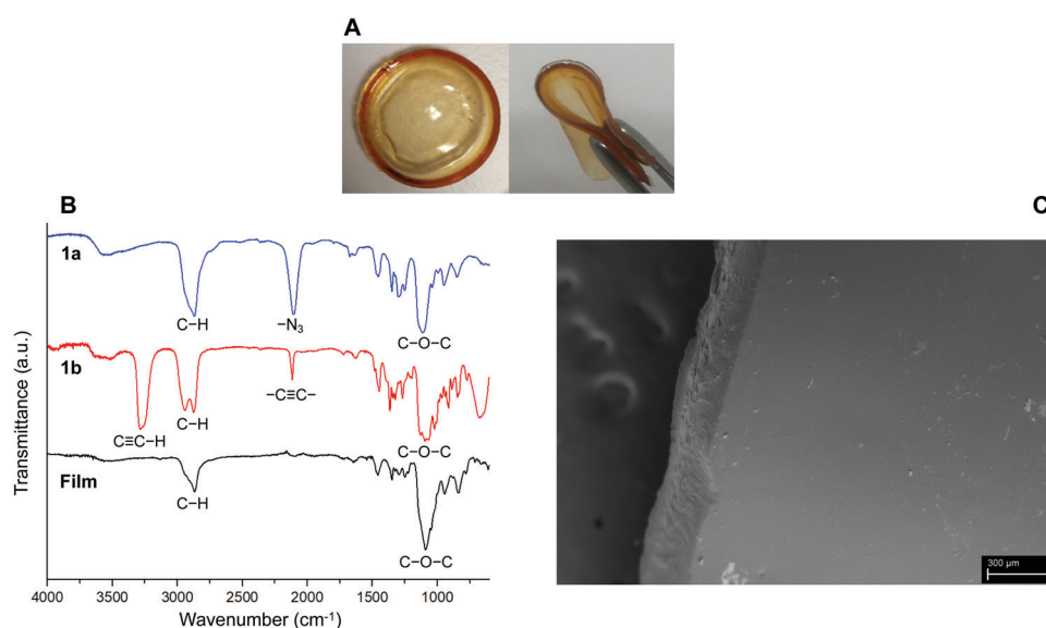
Fig. 1 (A) Digital images of obtained flexible hydrogel films (diameter of circular film = 4 cm). (B) FTIR spectra of 1a , 1b and the film. (C) SEM image of the hydrogel film. Scale bar = 300\text{ }\mu\text{m} .
