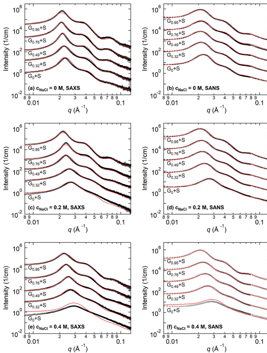
Fig. 3 SAXS and SANS profiles for 8 wt% G_x + S hydrogels at c_{\text{NaCl}} = 0, 0.2, and 0.4 M, where x denotes the molar percentage of the guanidinium moiety over total cations in the end-block of the triblock copolymer. Solid curves represent the best fit to the fitting model. Data and curves are vertically shifted for clarity.
