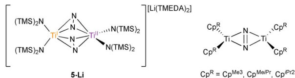
Fig. 4 Reported examples of bimetallic Ti complexes bridged by a side-on \text{N}_2 ligand. Left: double side-on \text{Ti}-(\text{N}_2)_2\text{-Ti} , 5-Li, complex. 26 Right: single side-on \text{N}_2 titanocene complexes. 5,7
