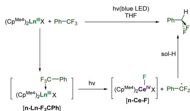
Scheme 2 General reaction scheme for C–F activation and hydrodefluorination by Ln complexes 1-Ln to 3-Ln and cleavage by the Ce photocatalysts 1-Ce – 6-Ce with \text{PhCF}_3 (X = the monoanionic ligand \text{Cp}^{\text{Me}_4} , Cl, OAr, OTf, Bn) n = 1-3 .
