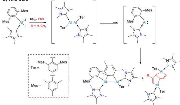
Scheme 1 (a) Examples of isolable Al(I) species (I–IX); and (b) synthesis of an arrested dialumene and deconstruction of arenes by a masked alumylene ( \text{Al}^{\text{I}} ) presented in this work.
