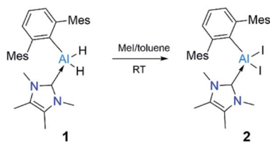
Scheme 2 Synthesis of compound 2. Mes = 2,4,6- \text{Me}_3\text{C}_6\text{H}_2 .
