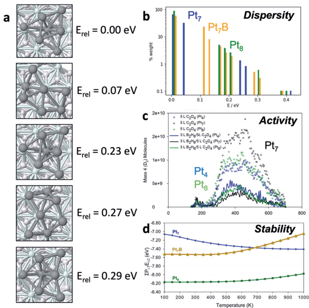
Fig. 1 (a) Isomers of \text{Pt}_7 supported on alumina. (b) Histograms showing the distribution of isomers for \text{Pt}_7 , \text{Pt}_7\text{B} and \text{Pt}_8 , on a log scale to improve visibility of high-energy low-weight isomers. Each bar shows the energy and 700 K population of one isomer. (c) Differences in catalytic activity of differently sized Pt clusters, as shown by temperature programmed desorption in the context of (deuterated) ethylene dehydrogenation. (d) Coking susceptibility of differently sized Pt clusters as a function of temperature.
