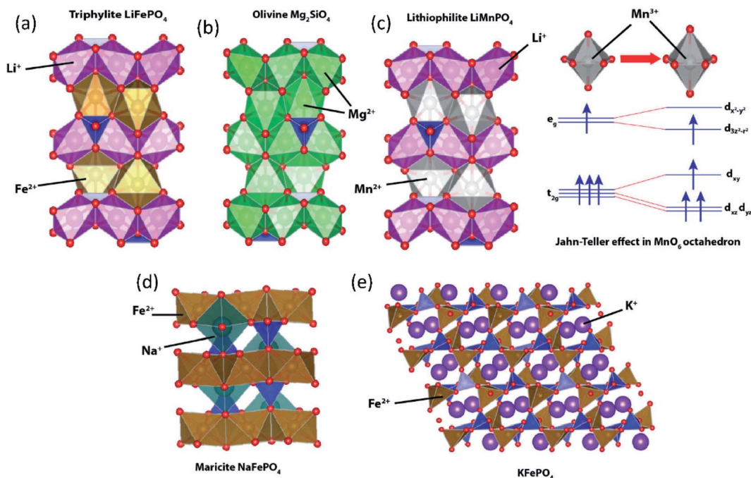
Fig. 9 Structural illustration of (a) triphylite LiFePO 4 , (b) olivine Mg 2 SiO 4 , (c) lithiophilite LiMnPO 4 with an inset showing Jahn–Teller distortion in MnO 6 , (d) maricite NaFePO 4 , and (e) KFePO 4 .
