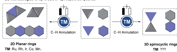
(c) Electrooxidative spiroannulation
