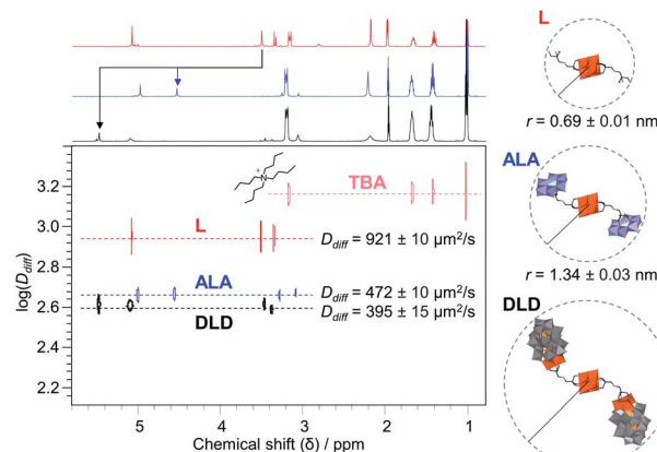
Fig. 6 Overlaid 1 H 2D DOSY NMR spectra of L, ALA and DLD labelled with the translational diffusion coefficient ( D_{diff} ) used to determine the hydrodynamic radius ( r ) for each structure, as shown on the right, and the corresponding 1 H 1D NMR spectra shown at the top.
