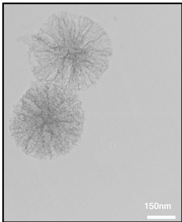
Fig. 12 TEM image of the recycled \text{Fe}_3\text{O}_4@\text{SiO}_2@\text{KCC}-1@\text{MPTMS}@Cu^{II} mesoporous nanocomposite.
