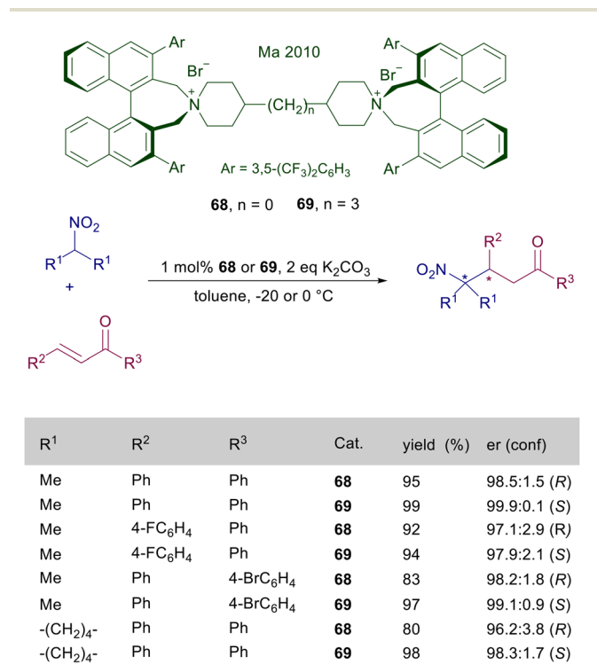
Scheme 51 Enantiodivergent conjugate addition of tertiary nitroalkanes to chalcones catalyzed by differently tethered ammonium salts 68 and 69 .
