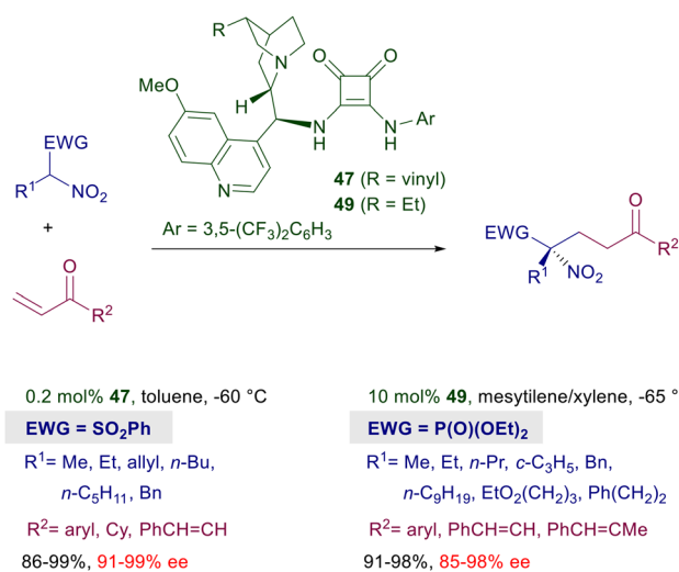
Scheme 37 Enantioselective conjugate addition of activated nitroalkanes to enones.
