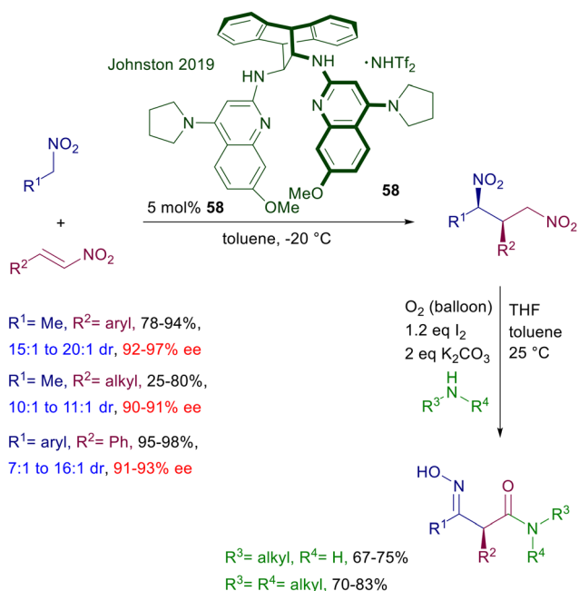
Scheme 42 Asymmetric synthesis of 3-hydroxyiminoalkenamides.
