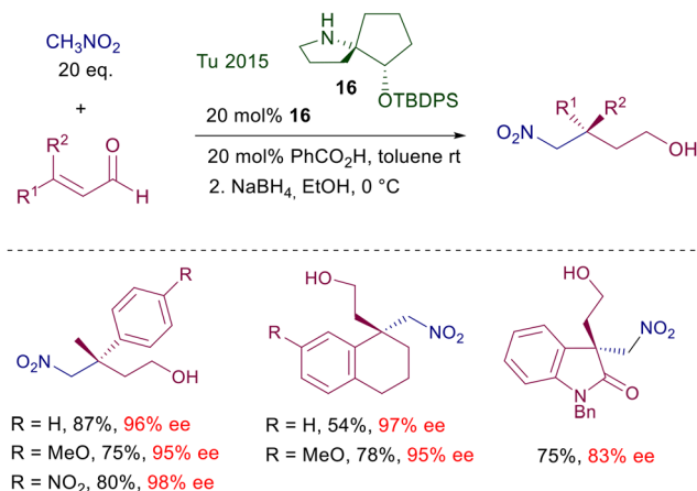
Scheme 10 Spiroprolinol embedding a silyl ether appendage.
