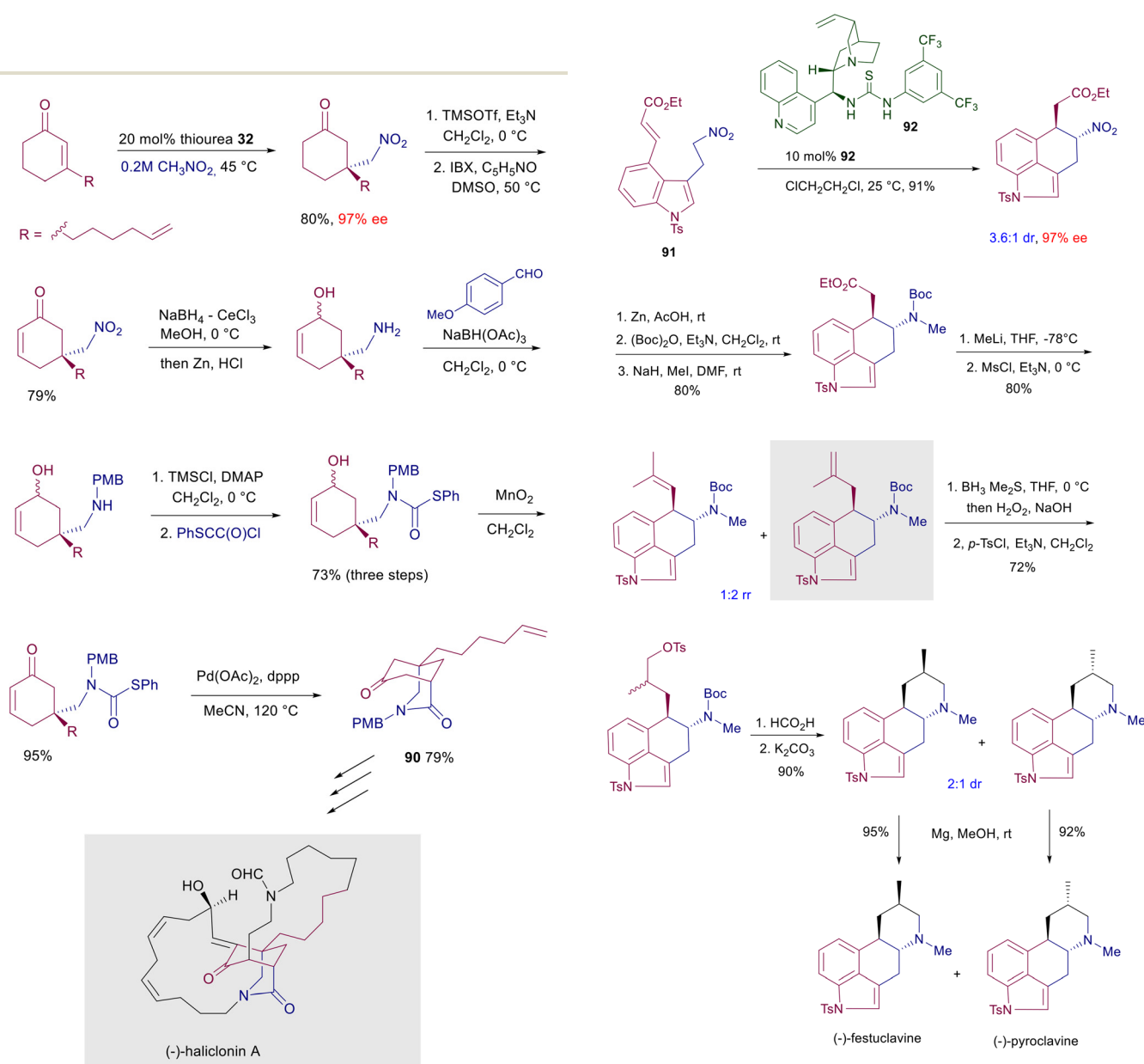
Scheme 69 Synthesis of the ergot alkaloids (–)-festuclavine and (–)-pyroclavine.
