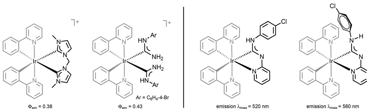
Fig. 4 (Left): structurally related luminescent \text{Ir}^{\text{III}} NHC and ADC complexes; 26,28 (right): conformers of \text{Ir}^{\text{III}} -ADC species showing distinct photo-physical properties. 49
