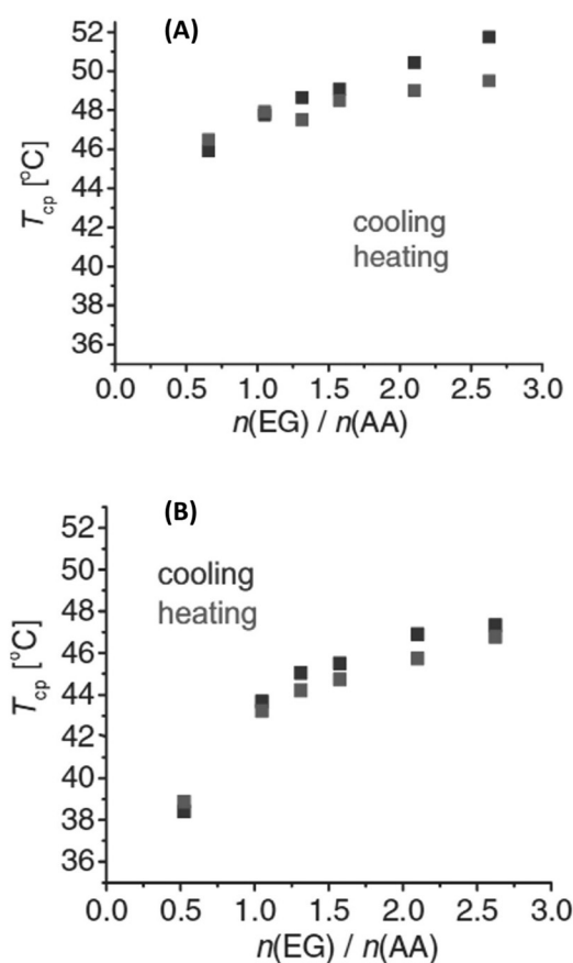
Fig. 13 Cloud point temperatures of (A) PEG/PAA and (B) PPEGMA/PAA solutions in iPrOH as a function of EG:AA monomeric unit molar ratios with 0.0625 \text{ wt\%} PAA concentration. Reproduced from ref. 113 Copyright 2017 WILEY-VCH Verlag GmbH & Co KGaA, Weinheim.
