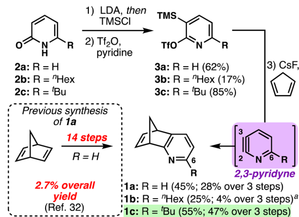
Fig. 2 Synthesis of pyridinonorbornenes 1a–c via 2,3-pyridynes. Reagents and conditions: (1) LDA (2.2 equiv.), THF, 0 °C, 1 h, then TMSCl (1.2 equiv.), 0 °C, 15 min, then rt, 12 h. (2) \text{TiF}_2\text{O} (1.1 equiv.), pyridine, 0 °C, 20 min, then rt, 12 h. (3) CsF (5.0 equiv.), \text{C}_5\text{H}_6 (5.0 equiv.), MeCN, 30 °C, 3 h. a 4 : 1 MeCN : DCM.
