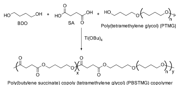
Scheme 17 Synthesis of poly[(butylene succinate)-co-poly(tetramethylene glycol)]s (PBSTMGs).
